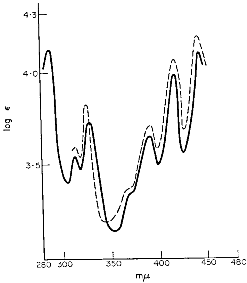
FIG. I. — Zinc dust distillation product of xylindein --- peri -Xanthenoxanthene
