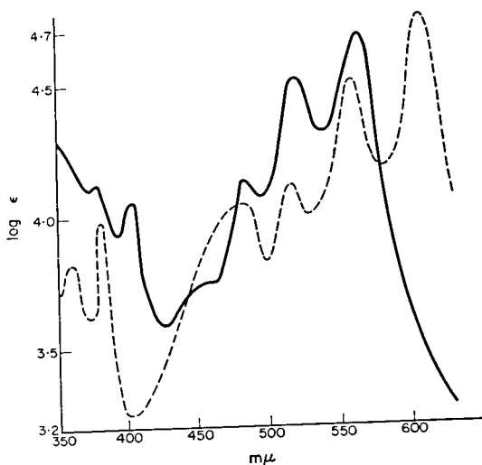
FIG. III. — Dimethylxylindein --- peri -Xanthenoxanthene-4,10-quinone
