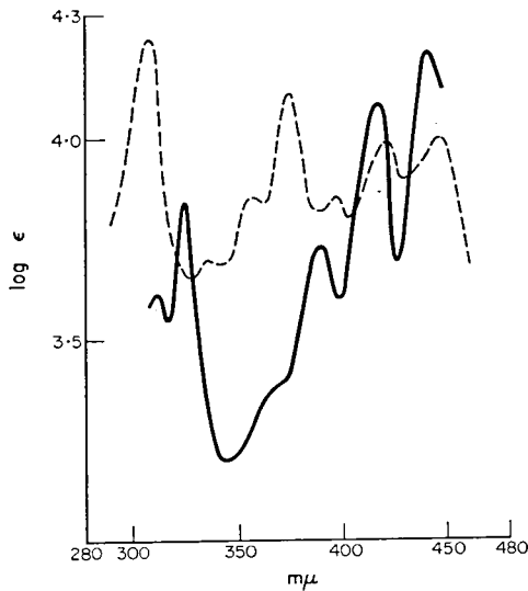
FIG. II. — peri -Xanthenoxanthene --- Dihydro-tetra-acetylxylindein
